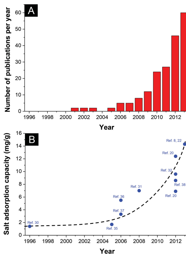
Figure 1. A) Number of publications per year for capacitive deionization and B) development of NaCl electrosorption capacity reported for electrodes made of carbon materials (values and parameters are outlined in Table 1).
